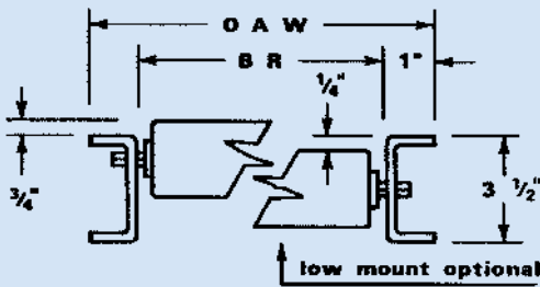
2-1/2" Medium Duty Roller Conveyor
